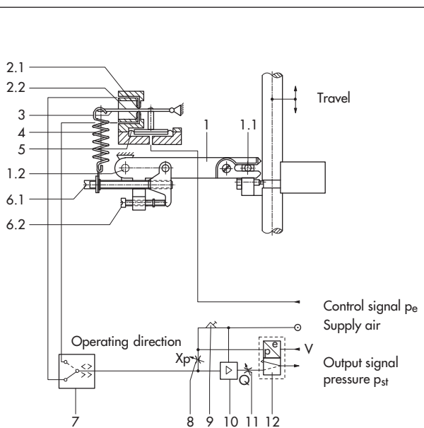
Fig. 6 · Functional diagram of Type 3766 Positioner (deflection of pick-up lever in case of direct attachment to Type 3277 Pneumatic Actuator)
